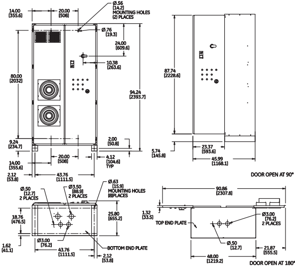
150-300 HP@460V & 150 HP@575V
