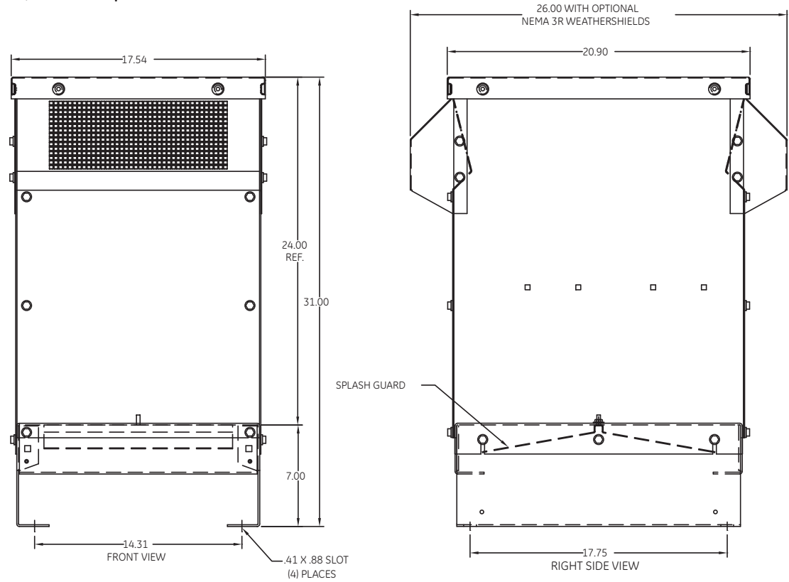
CAB-17C, 52-103 Amps
